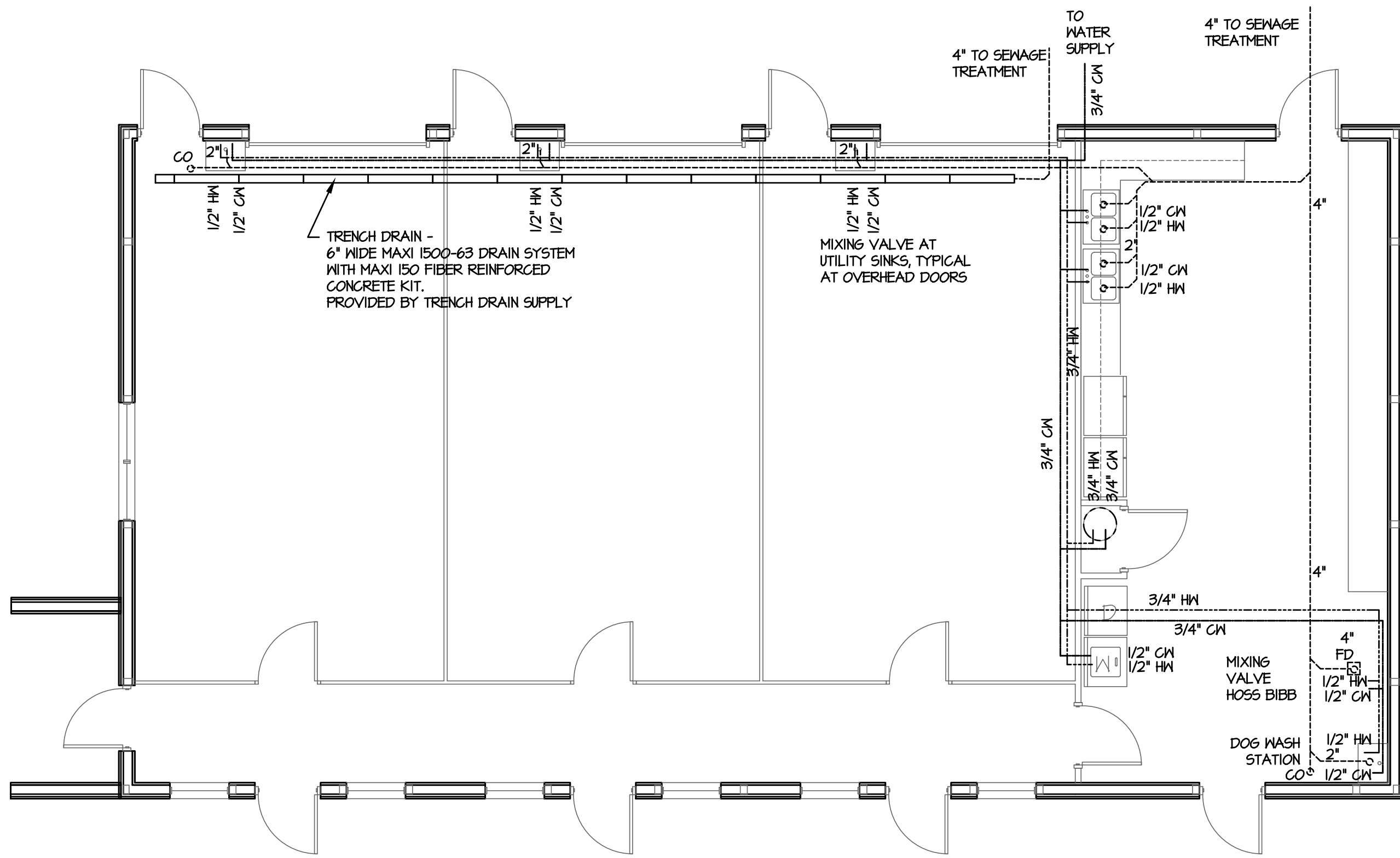
1 PLUMBING PLAN 3/16" = 1'-0"
