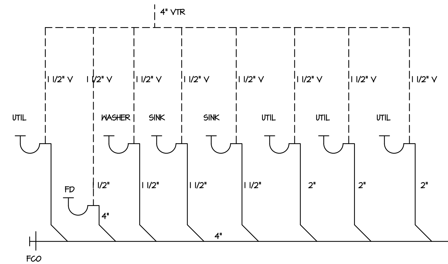
3 SANITARY RISER DIAGRAM NO SCALE
