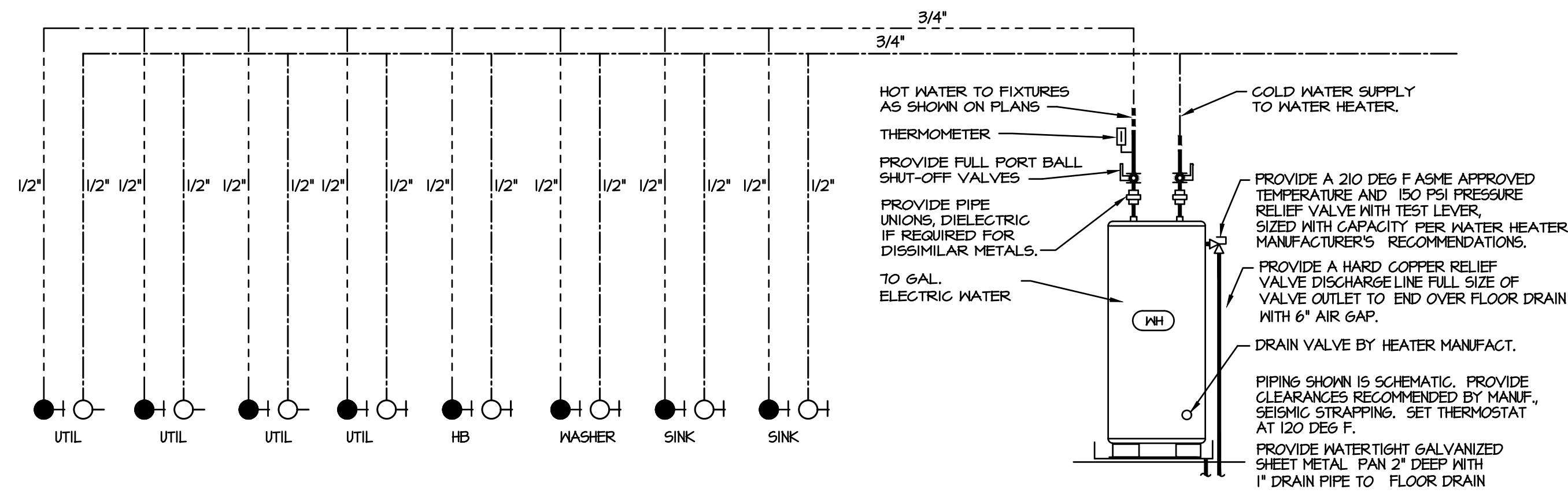
2 SUPPLY RISER DIAGRAM NO SCALE
