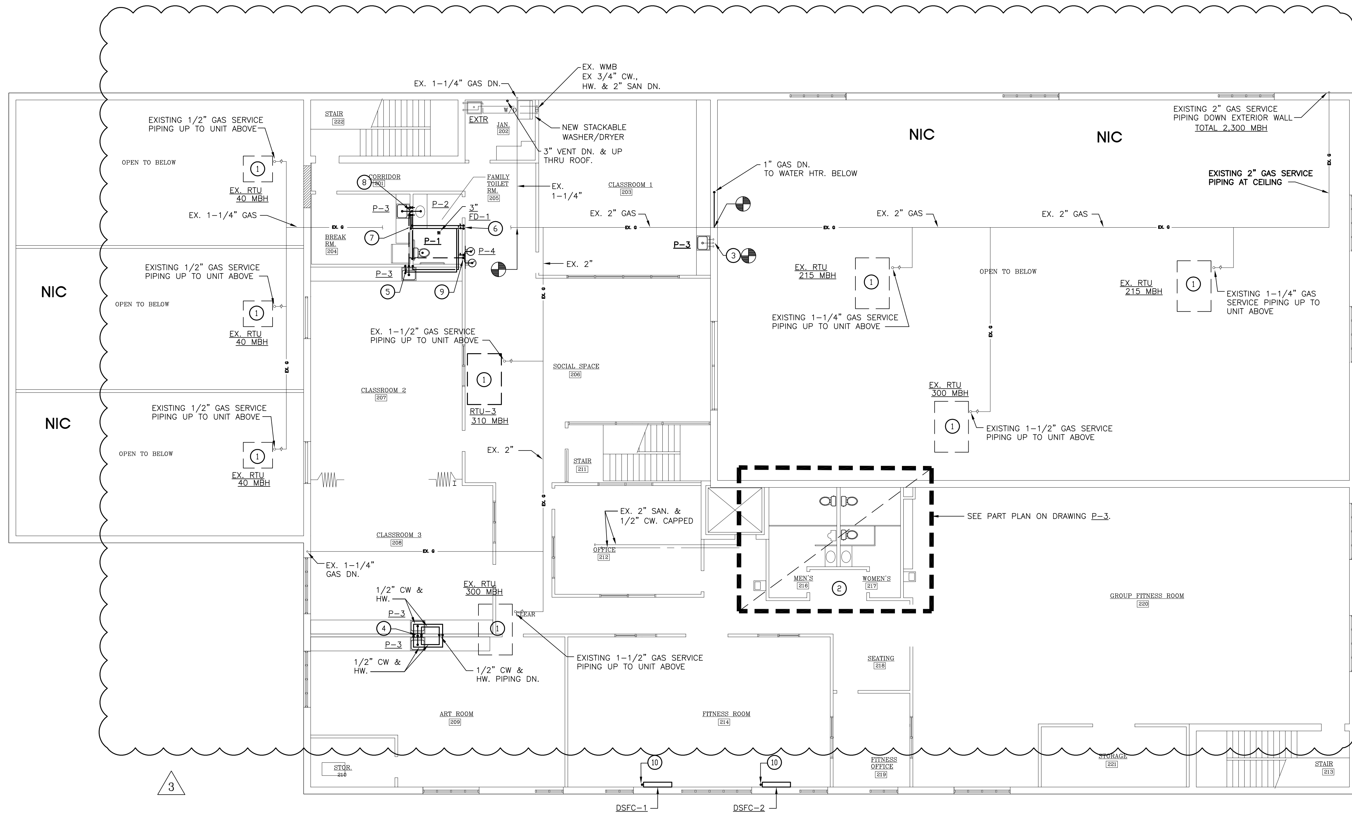
SECOND FLOOR PLAN - PLUMBING NEW WORK SCALE: 1/8"=1'-0"
