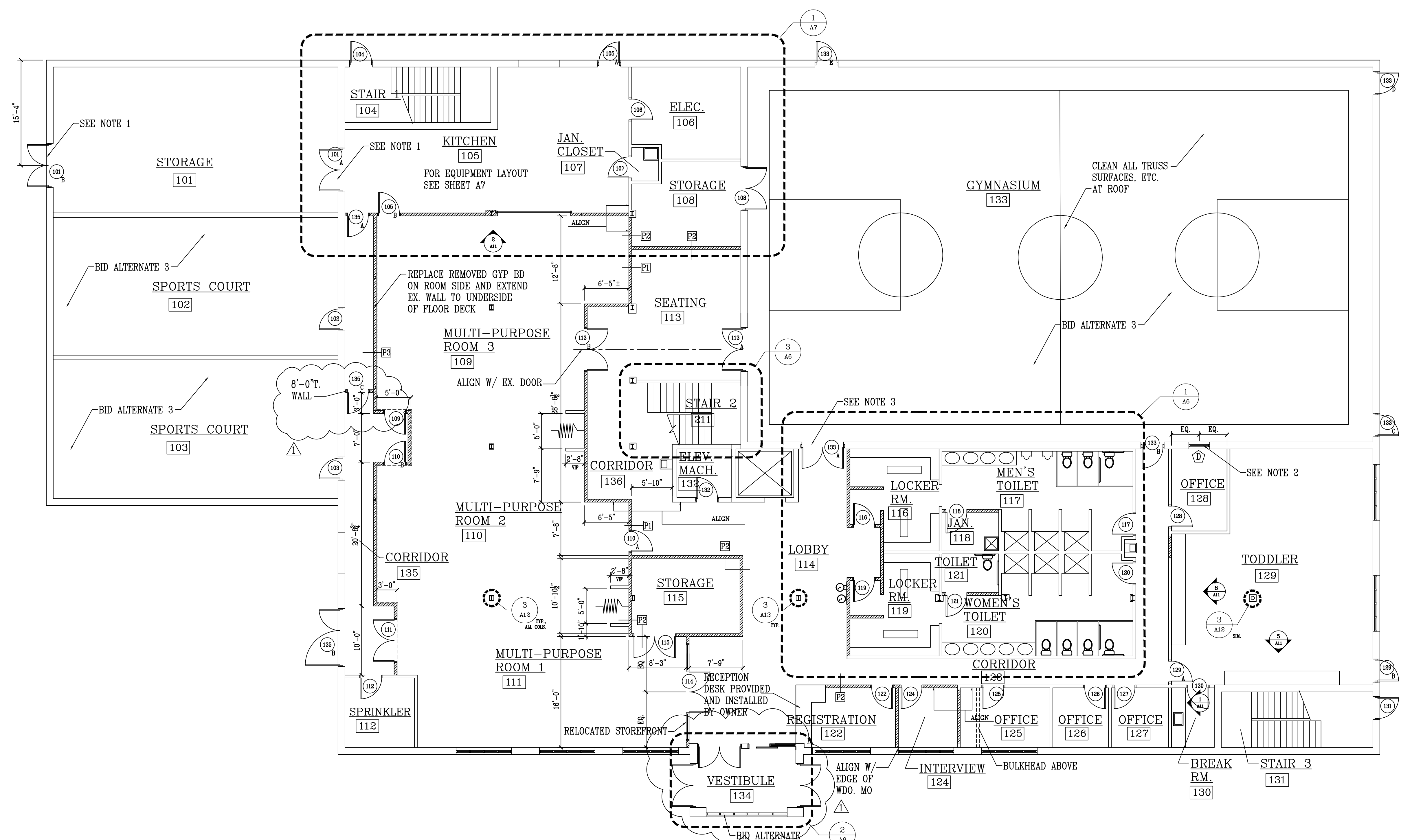
1 COMPOSITE PLAN - FIRST FLOOR 1/8" = 1'-0"
