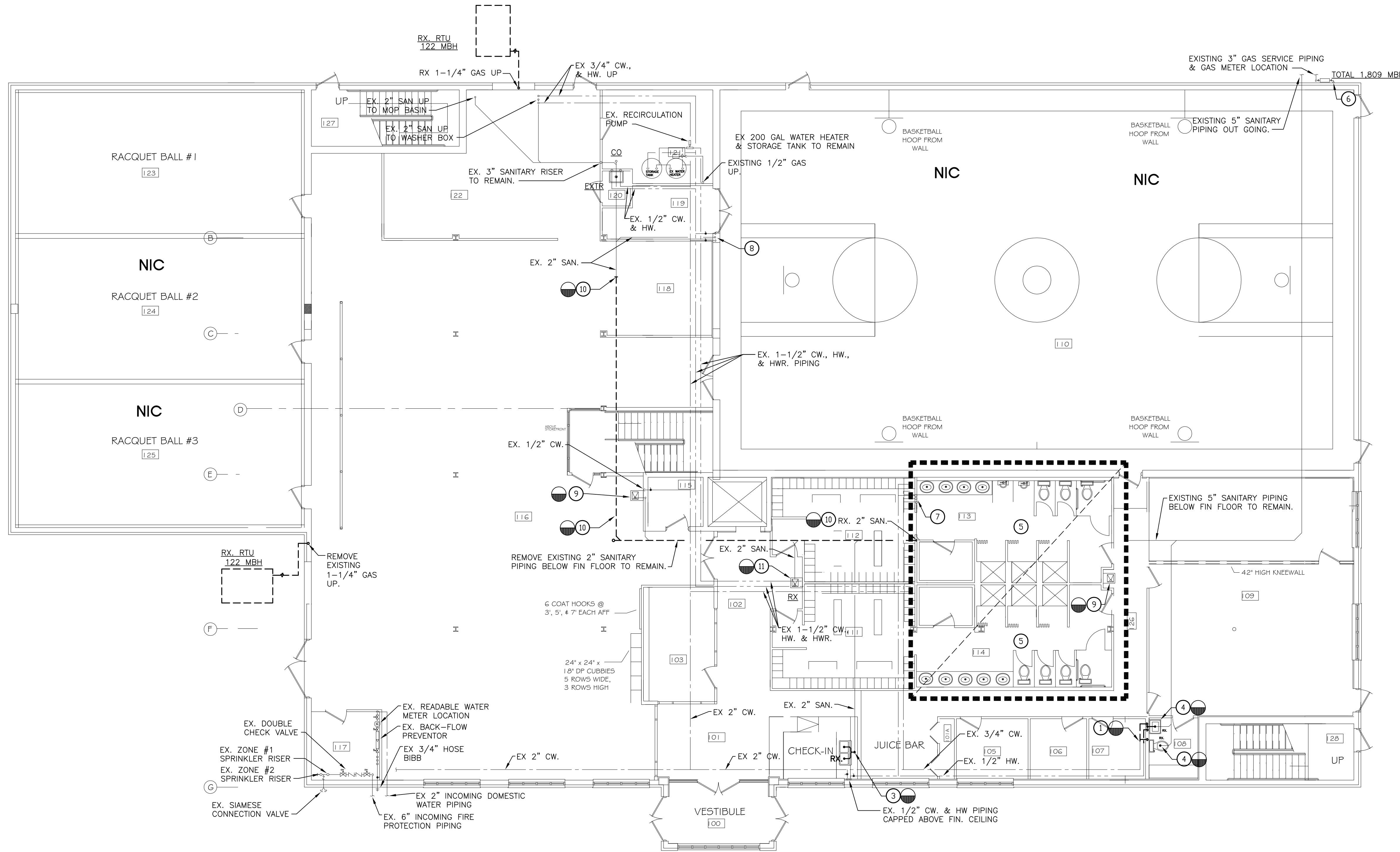
FIRST FLOOR PLAN - PLUMBING DEMOLITION SCALE: 1/8"=1'-0"
