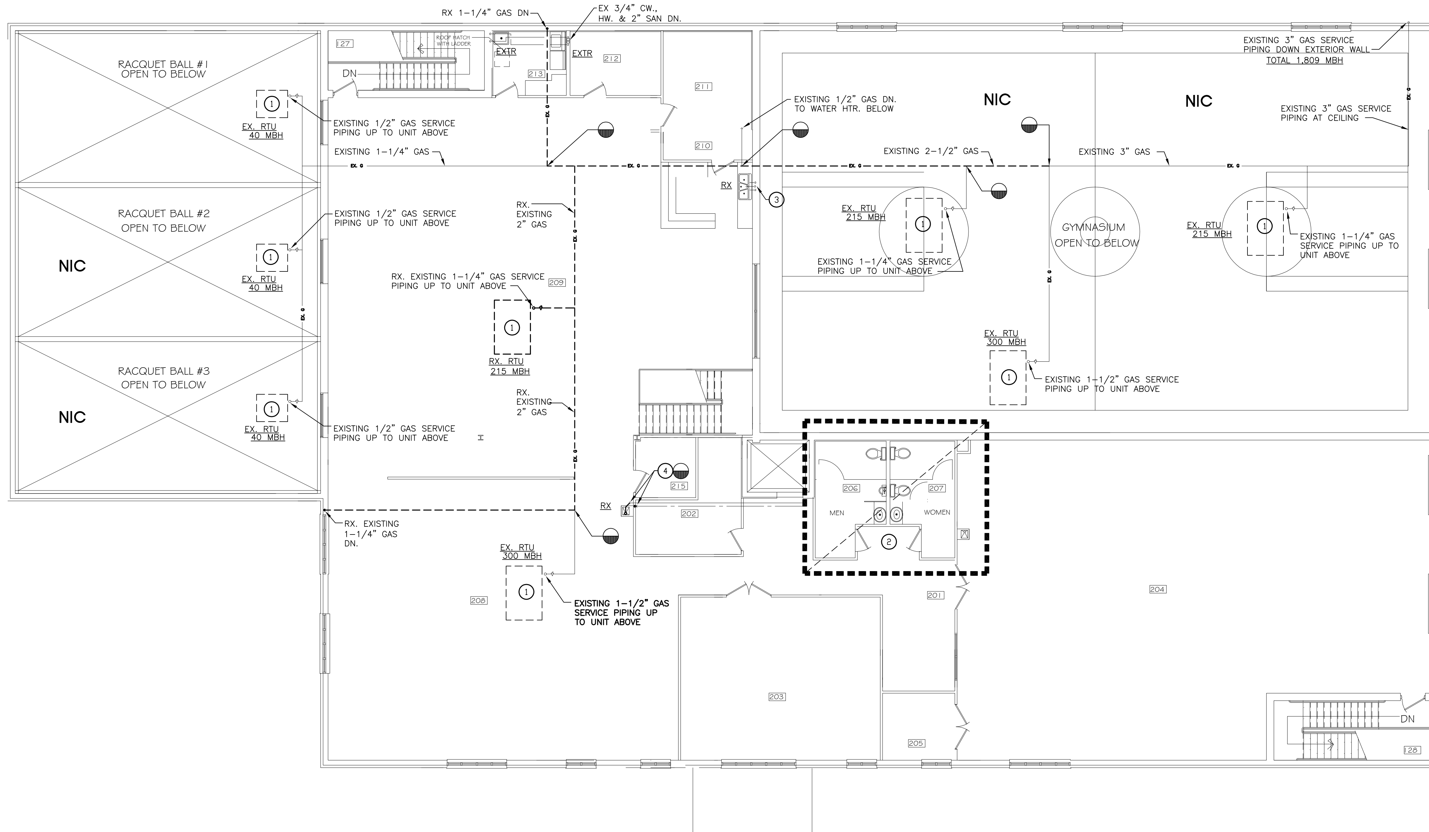
SECOND FLOOR PLAN - PLUMBING DEMOLITION SCALE: 1/8"=1'-0"
